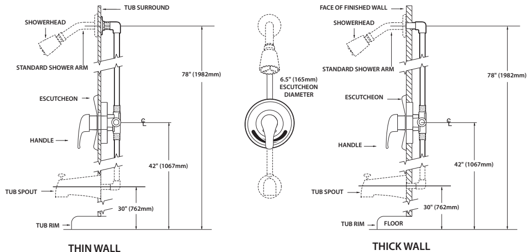
THIN WALL
